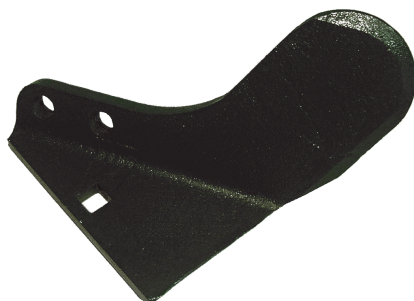
#010M Cast Manganese Alloy Nose Piece (MTO Spec. ES-507)
