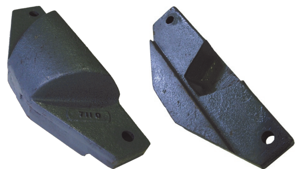
#7110 Wing Shoe Grey Iron Casting, 12" hole centres
